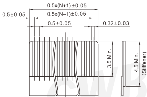
APPLICABLE TCP RECOMMENDED DIMENSION (THICKNESS : 0.12 ± 0.03)
