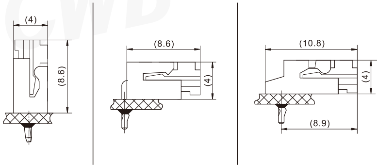
Assembly View (DIM FYI)
