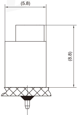
Assembly View (DIM FYI)
