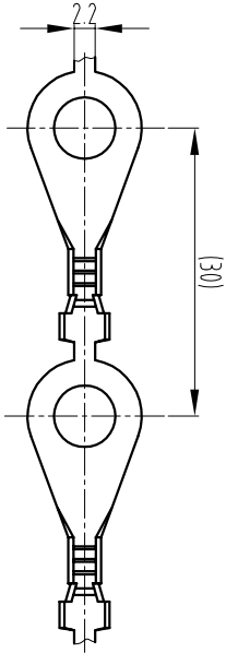
Contact View 1:2
