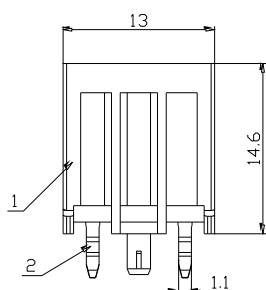
TJC79201-2AD 插头 Plug Connector
