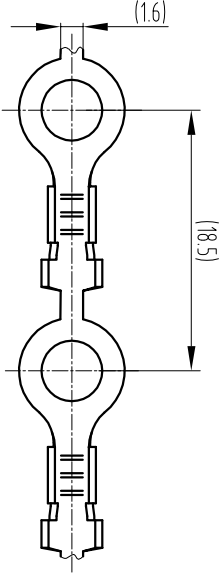
Contact View 1:2
