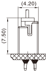
Assembly View (TJC15014-nADK&TJC15014-nY) (FYI)
