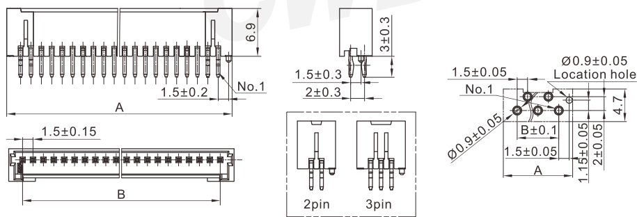
PCB Layout
