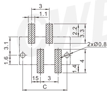
PCB Layout
