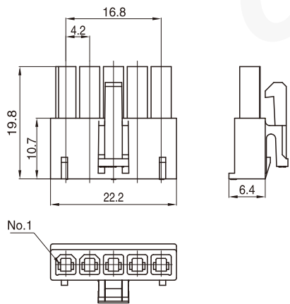
孔座 (含锁紧片保持结构) Housing (W/Retainer)
