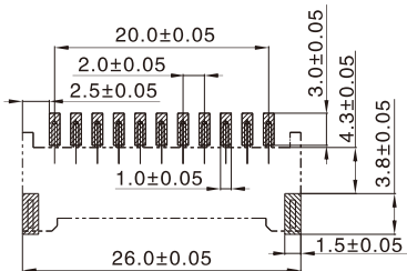
PCB Layout (FYI)
