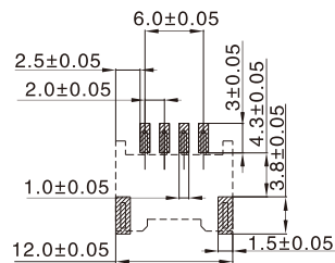
PCB Layout (FYI)
