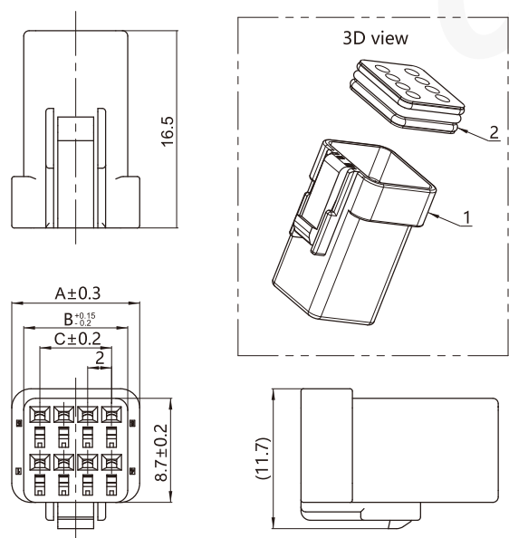
孔座组装件 Plug housing Assy
