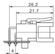
Assembly View (DIM FYI)
