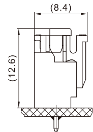
Assembly View (DIM FYI)
