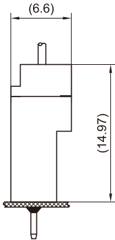
Assembly View (DIM FYI)
