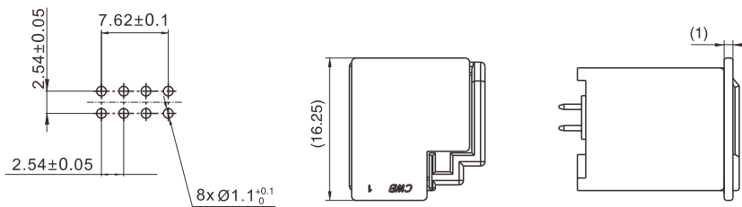
PCB Layout
