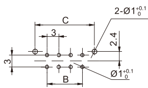
PCB Layout
