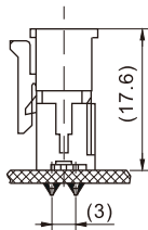
Assembly View (DIM FYI)
