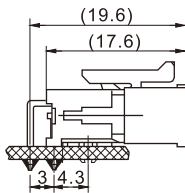
Assembly View (DIM FYI)
