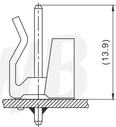
Assembly View (DIM FYI)
