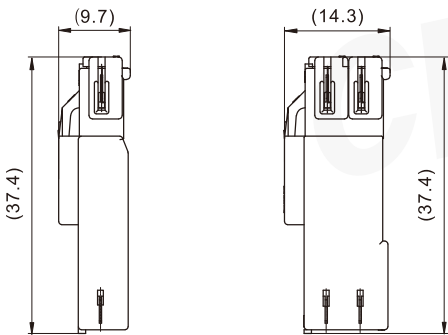
Assembly View (DIM FYI)
