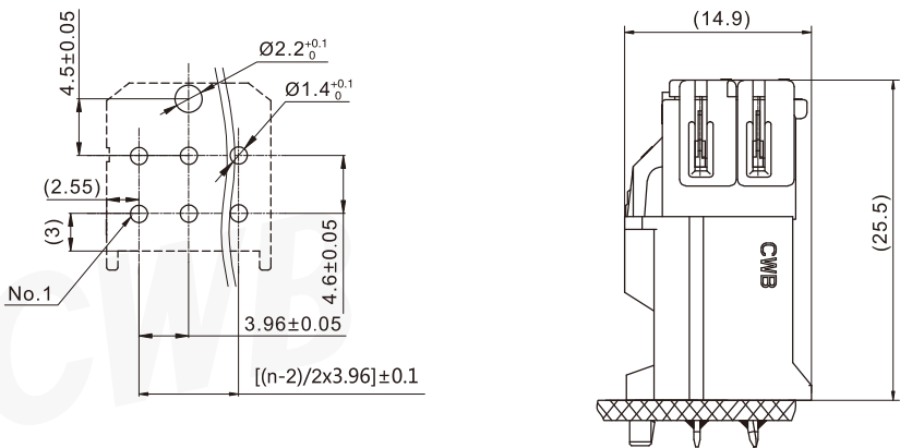
PCB Layout
