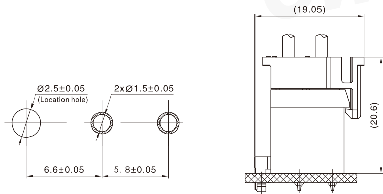
PCB Layout
