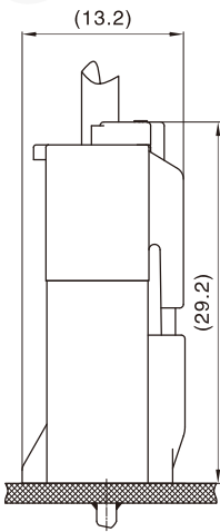
Assembly View (TJC6203-nY&TJC6203-nA) ( FYI )
