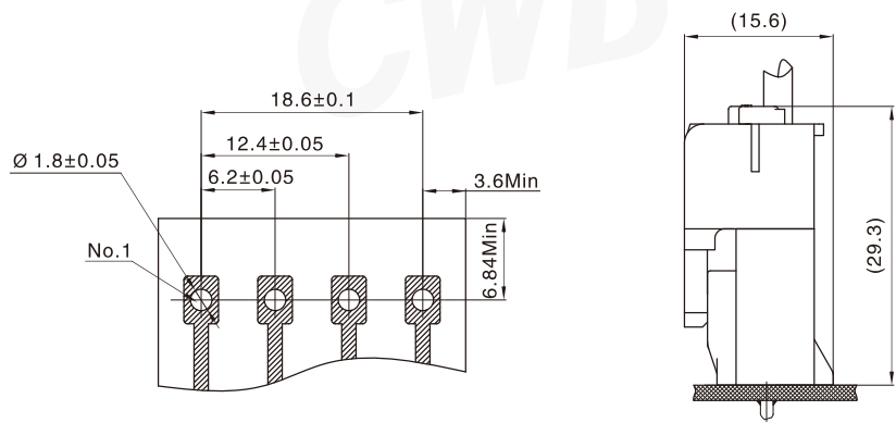
PCB Layout
