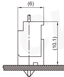
Assembly View (DIM FYI)
