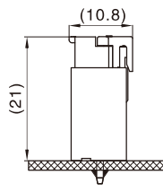
Assembly View (VH-nAD&VHB-2~4Y) (FYI)
