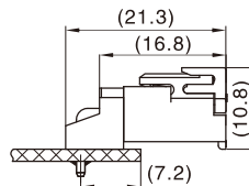
Assembly View (VH-nAD&VHB-2~4Y) (FYI)
