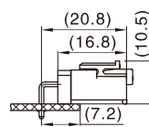
Assembly View (VH-5~7AW&VHB-5~7Y) (FYI)
