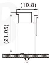
Assembly View (VH-nAWJ&VH-nY) (FYI)
