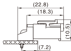
Assembly View (VH-nAD&VHB-5~7Y) (FYI)
