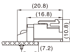
Assembly View (VH-nAW&VH-nY) (FYI)
