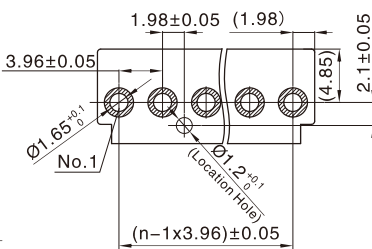
VH-3AD~9AD PCB Layout
