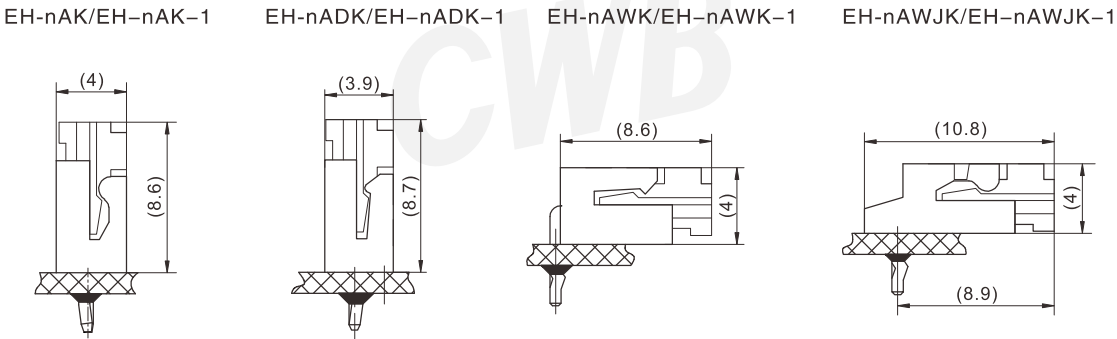
Assembly View (DIM FYI)
