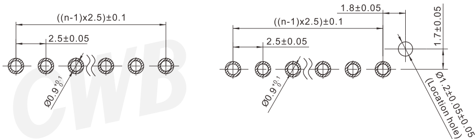
EH PCB Layout
